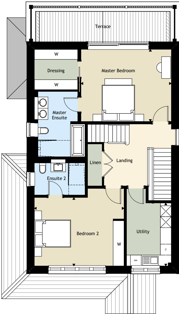
First Floor
